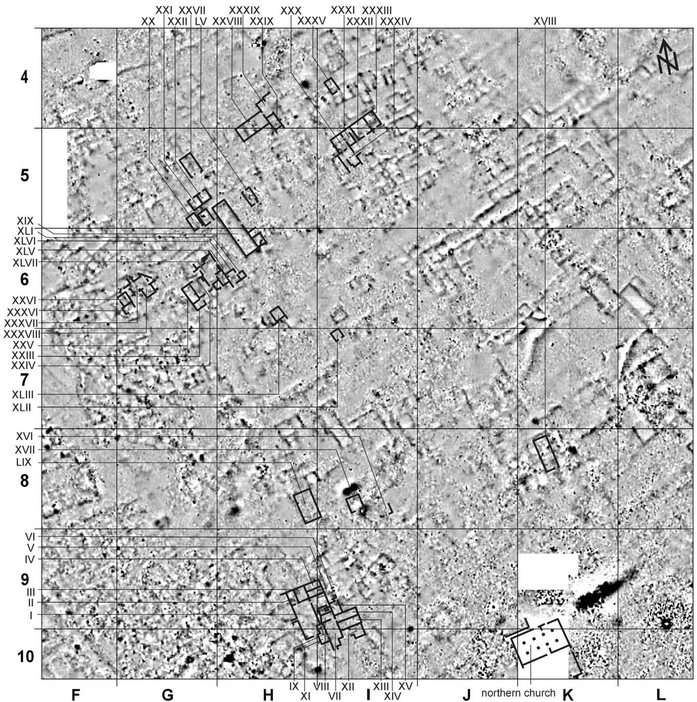
FIG. 15. Magnetic map of the northern part of the kom with superimposed features from Golvin's map (northern group situated in relation to room XIX, southern in relation to the northern church). Numerical and letter coordinates on the axes follow fig. 12. Dynamics: -2.7 nT (white) / +7.4 nT (black). Grid lines every 40 m. Map by T. Herbich.
