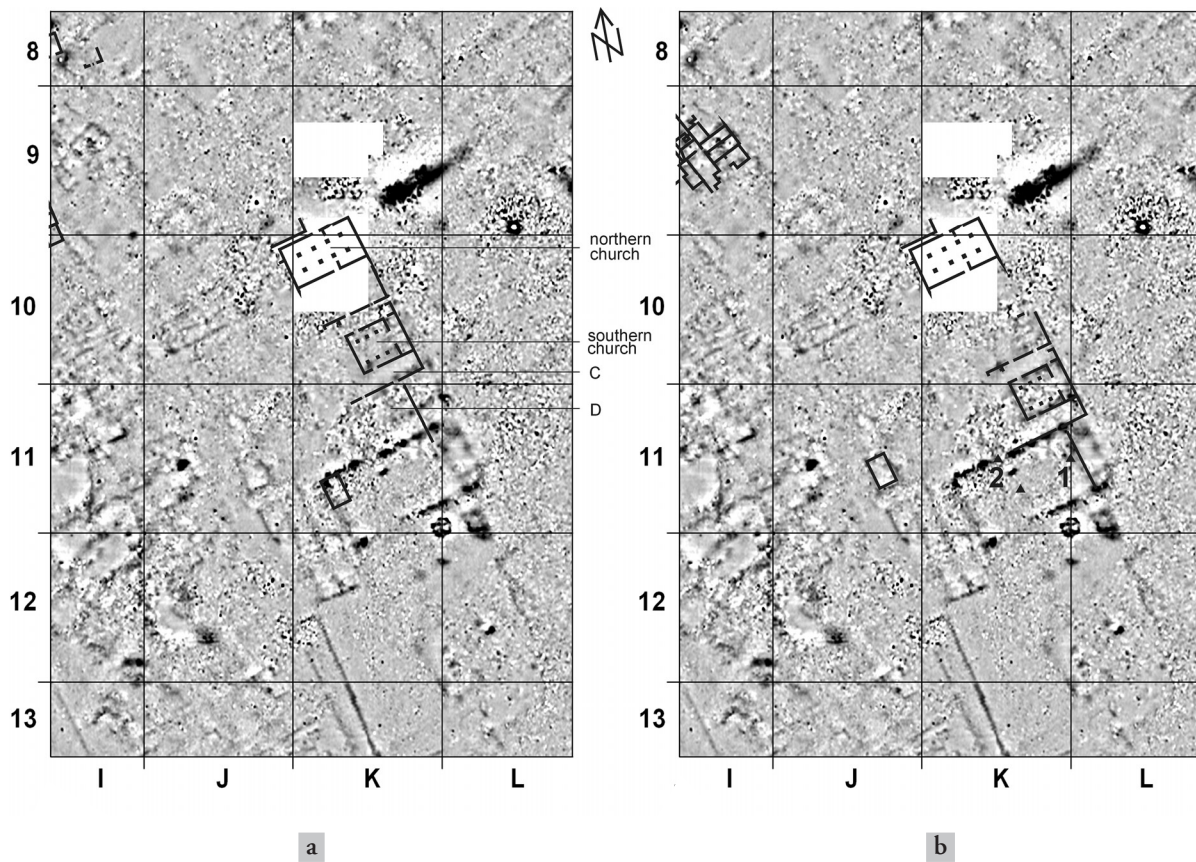
FIG. 18. Magnetic map of the area of the northern and southern churches. Dynamics: -3.4 nT (white) / +9.7 nT (black). Grid lines every 40 m. Numerical and letter coordinates on the axes follow fig. 12.
