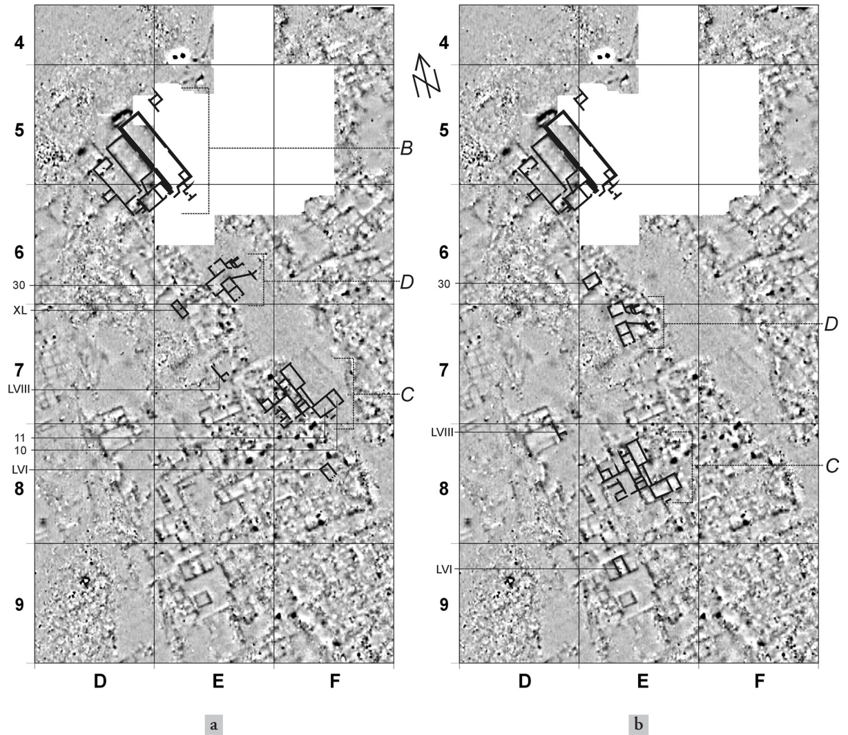
FIG. 17. Magnetic map of the northern part of the kom (area of Maspero's excavations). Dynamics: -2.7 nT (white) / +7.4 nT (black). Grid lines every 40 m. Numerical and letter coordinates on the axes follow fig.12. a) Features superimposed on the magnetic map following arrangement from Golvin's map; b) Feature localization based on analysis of magnetic map. Map by T. Herbich.
