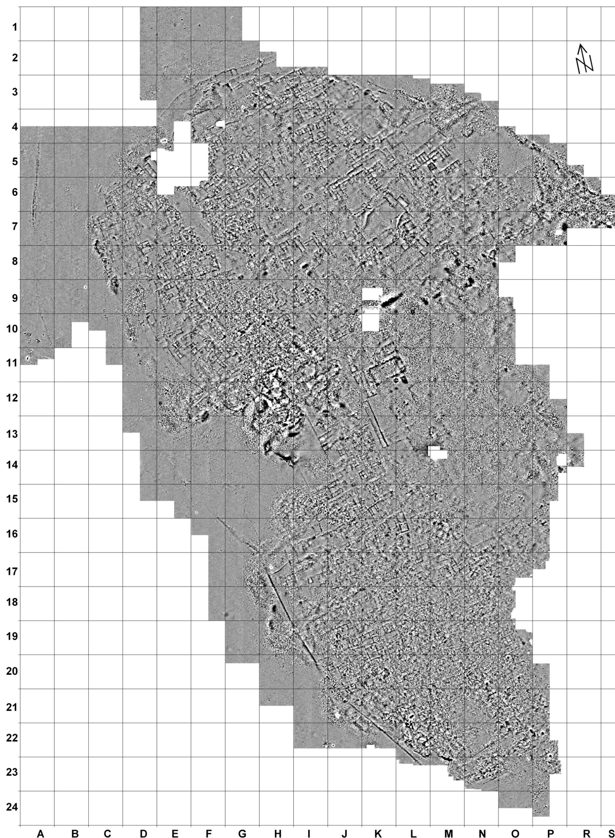
FIG. 12. Magnetic map. Survey 2004-2007. Geoscan Research gradiometers FM18, 36 and 256. Sampling grid 0.25 \times 0.50 m interpolated to 0.25 \times 0.25 m. Low pass filter. Dynamics: -3 nT (white) / +5 nT (black). Grid lines every 40 m
