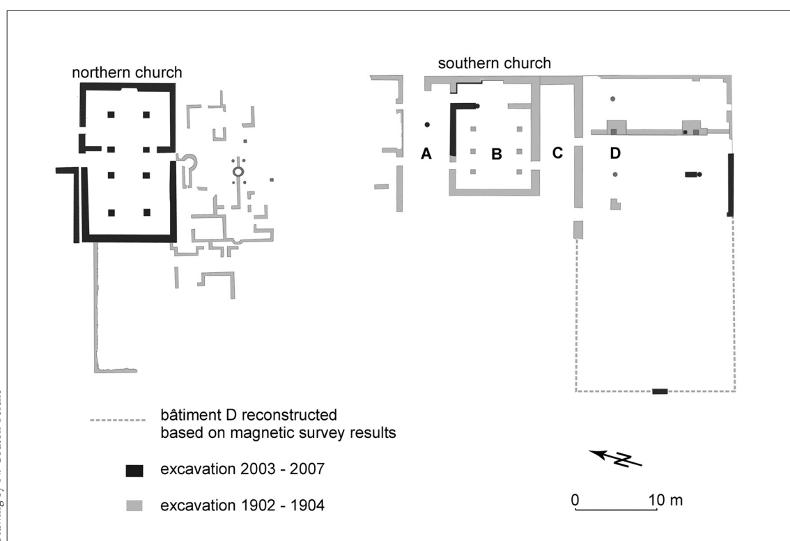
FIG. 20. Reconstruction of the plan of the church complex based on documents 3, 6, 8, 9, results of excavation 2003-2007 and results of magnetic survey.
