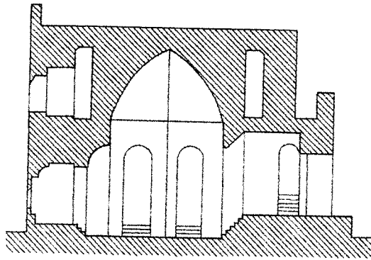
SECTION (RECONSTRUCTION)
