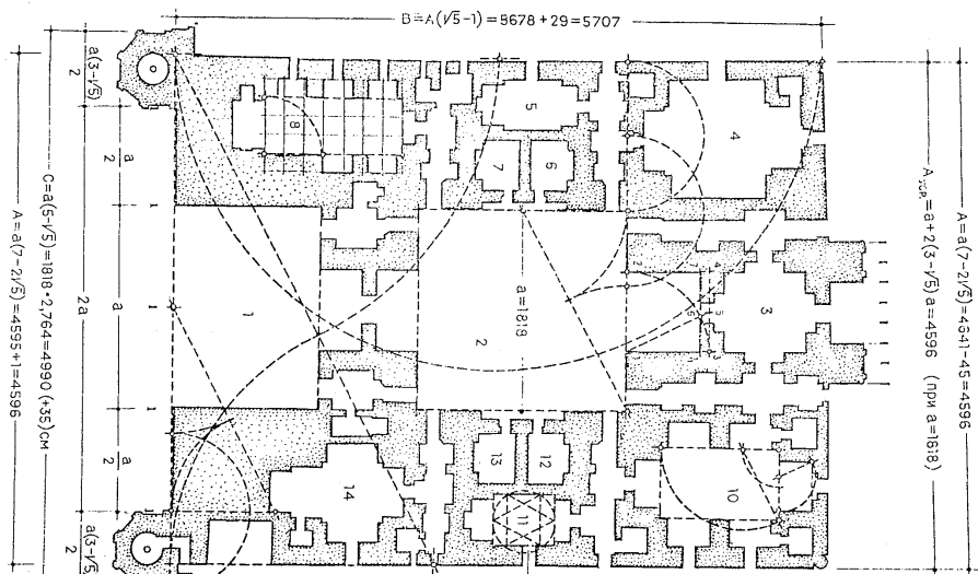
c. Turkistan, Shrine of Ahmad Yasavi, 1397-1399, geometric analysis of ground plan (after Bakhlov).
