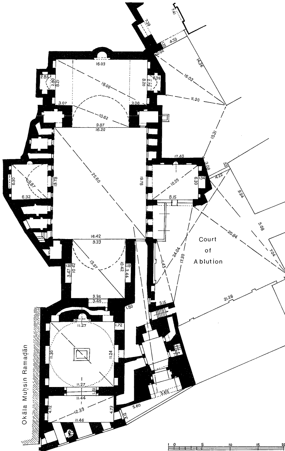
Fig. 9. — Ḥānqā of Baybars al-Ġāšankir. Plan [Source : K.A.C. Creswell, The Muslim Architecture of Egypt (Oxford : The Clarendon Press, 1952-59) fig. 142].
