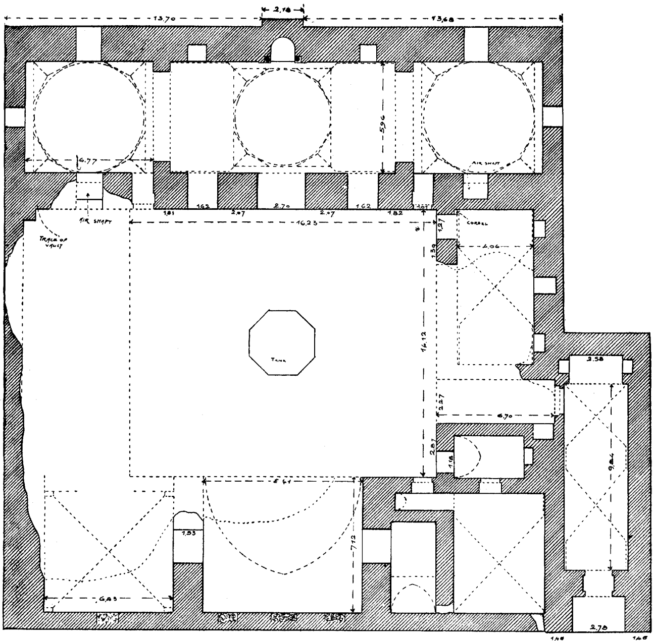
Fig. 8. — Kāmiliya Madrasa, at Aleppo (Firdaus).
