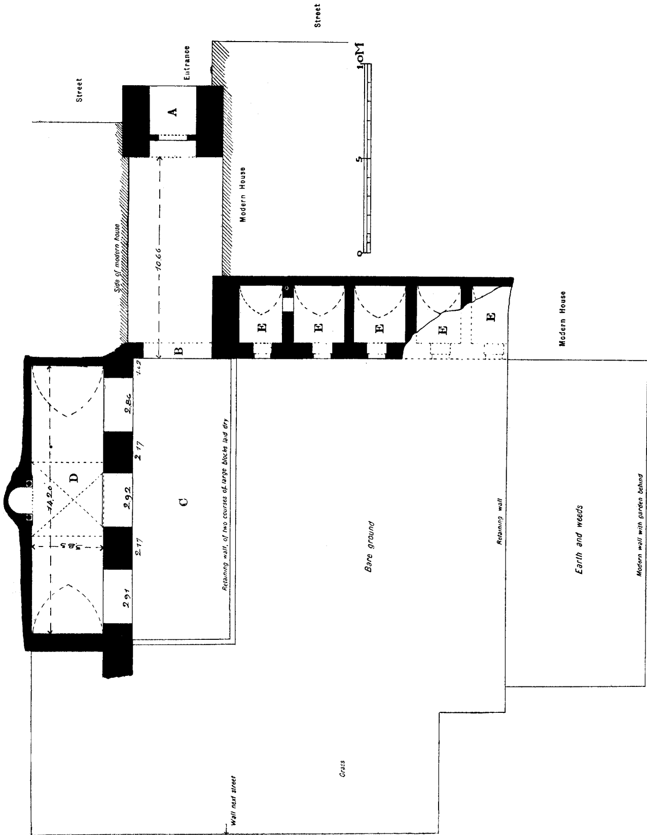
Fig. 1. — Madrasa Khan at-Tūtūn, at Aleppo.
