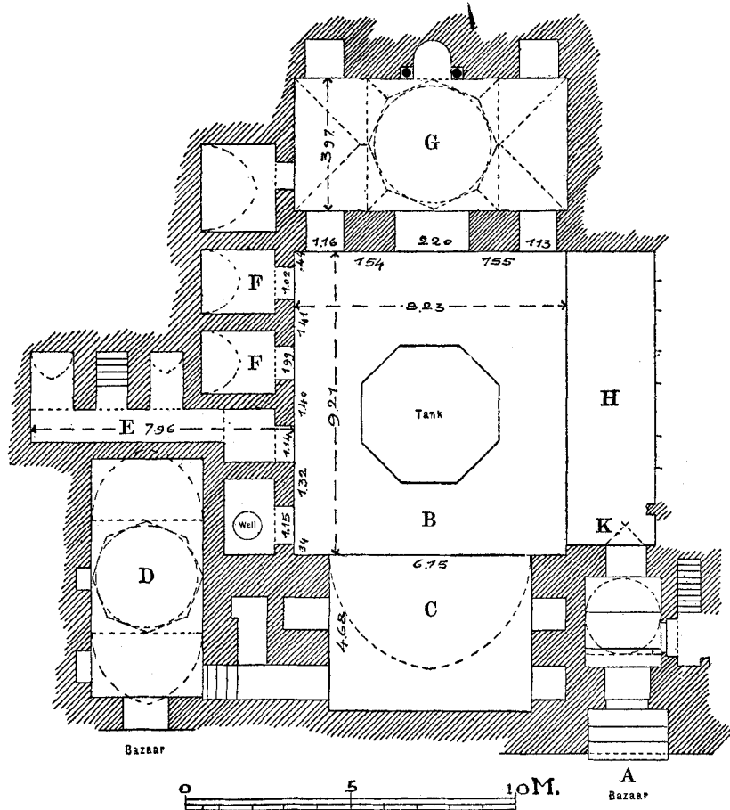
Fig. 2. — Madrasa of the Emir Shād Bakht, at Aleppo.
