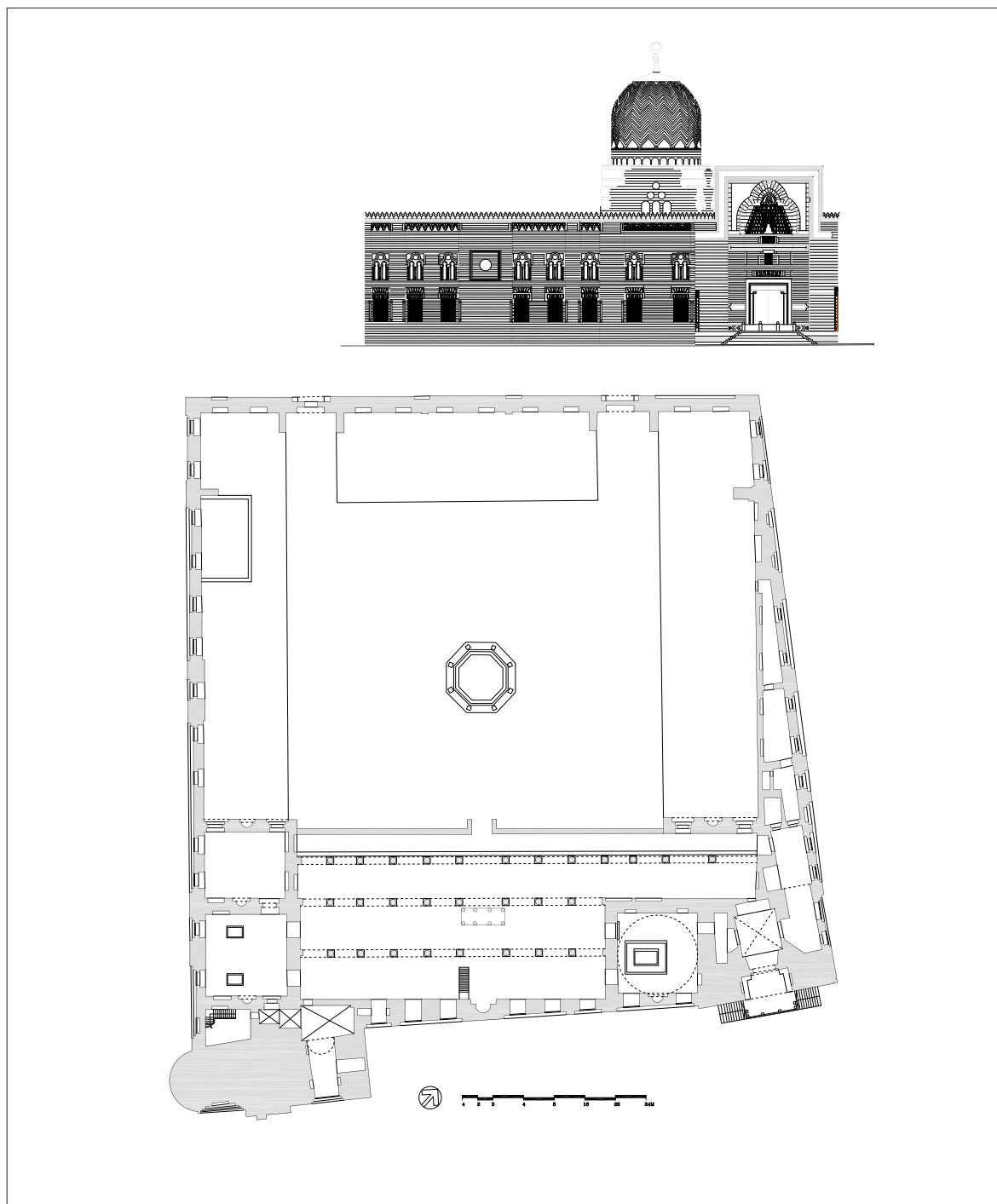
Fig. 1. Main façade and ground plan of the mosque of al-Mu'ayyad Šayḥ near Bāb Zuwayla.
